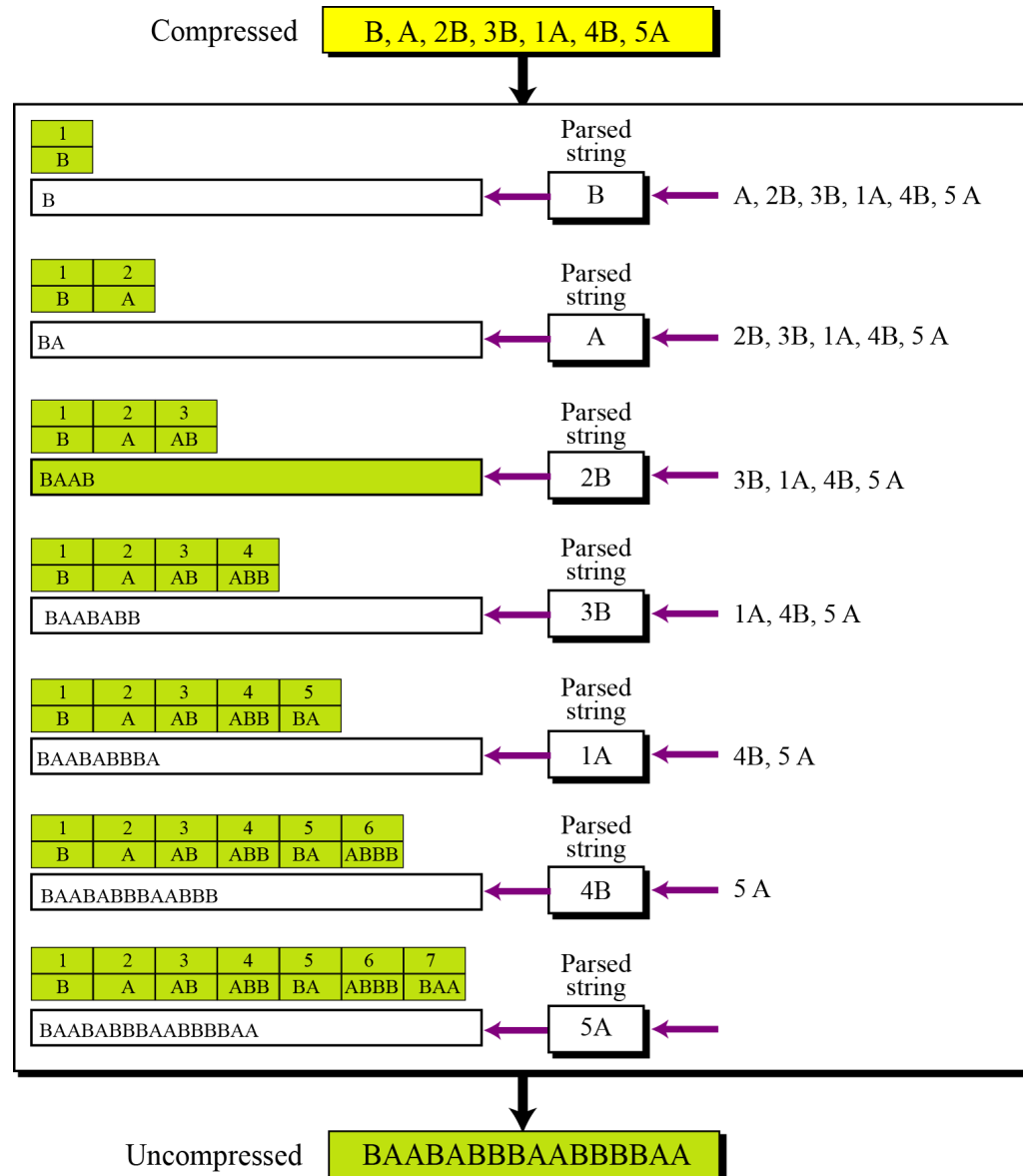
Figure 9 An example of Lempel Ziv decoding
